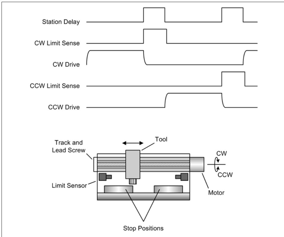
Figure 9-21. Sequentially controlled robotic system
